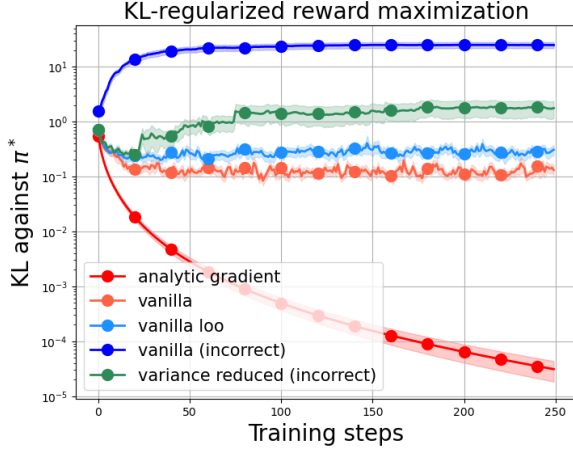
Figure 4. Measuring the KL divergence between \pi and optimal policy \pi^* for KL-regularized maximization problems. We initialize \pi = \pi_{\text{ref}} and follow the gradient estimates that combine the reward and KL components. While vanilla estimates generally decrease \mathbb{KL}(\pi, \pi^*) converging to a value that depends on the sample size, the incorrectly implemented vanilla and variance reduced estimates do not.
