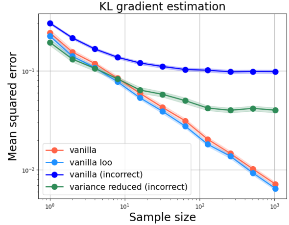
Figure 2. Comparing the accuracy of KL gradient estimation. We label biased implementations as incorrect . As sample size increases, vanilla estimates obtain lower MSE while estimates resulting from incorrect implementations plateau at large MSE due to bias . The vanilla estimate with leave-one-out control variate obtains marginally smaller variance . In RL for LLM, we find that proper KL gradient estimates make significant difference when the KL divergence is large, e.g., for on-policy distillation .
