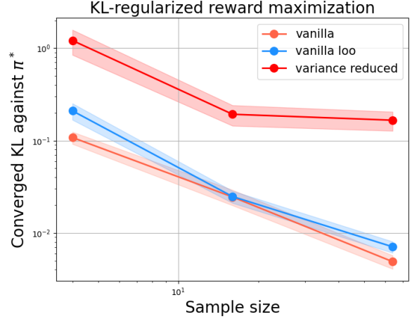
Figure 5. The converged value of \mathbb{KL}(\pi, \pi^*) as a function of the sample size. As sample size increases, vanilla gradient estimates obtain lower error values. However, the incorrectly implemented variance reduced estimate plateaus at a higher error.
