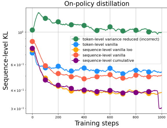
Figure 8. On-policy distillation of a 70B policy \pi_{\text{ref}} into a 8B policy \pi by minimizing KL divergence. To compare token-level losses, the vanilla gradient estimate minimizes the target metric, while the variance reduced estimate does not. Furthermore, proper sequence-level implementations minimize the KL at faster rate, with significant impact from variance reduction techniques.
