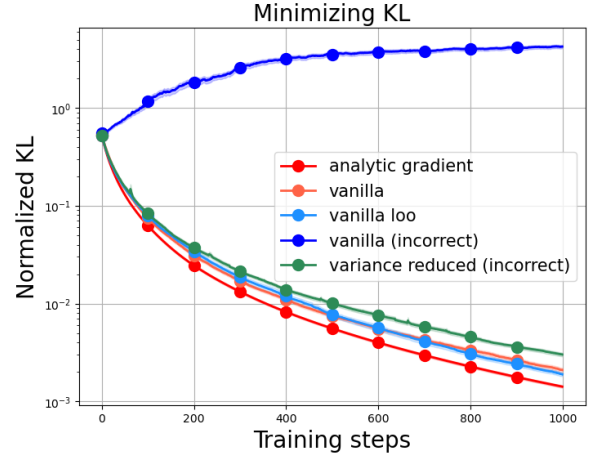
Figure 3. Comparing the efficacy of different estimates at minimizing KL divergence in tabular settings. We initialize \pi to be different from \pi_{\text{ref}} and descend on the KL gradient estimate. Except the incorrectly implemented vanilla estimate, which has zero expected gradient, other estimates generally decrease the KL divergence.
