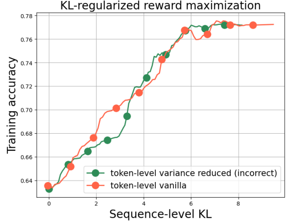
Figure 7. KL-regularized reward maximization with 8B models. Different estimates behave similarly in the low-KL regime, where enforcing different divergences lead to similar performance-KL trade-off.
