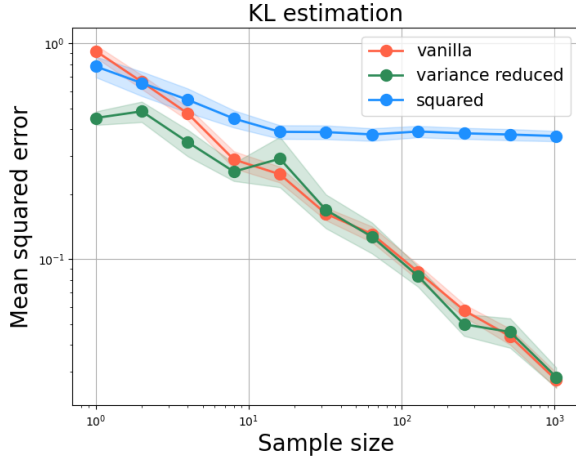
Figure 1. Comparing the accuracy of KL divergence estimation. At small sample size , variance reduced and squared estimates have lower mean squared error (MSE) compared to vanilla thanks to lower variance. At large sample size , squared estimate underperforms due to bias.
